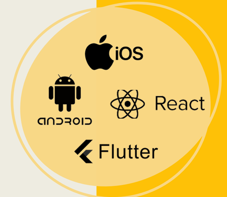
Mobile Apps
