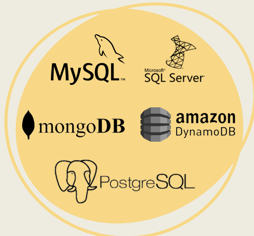
Databases
